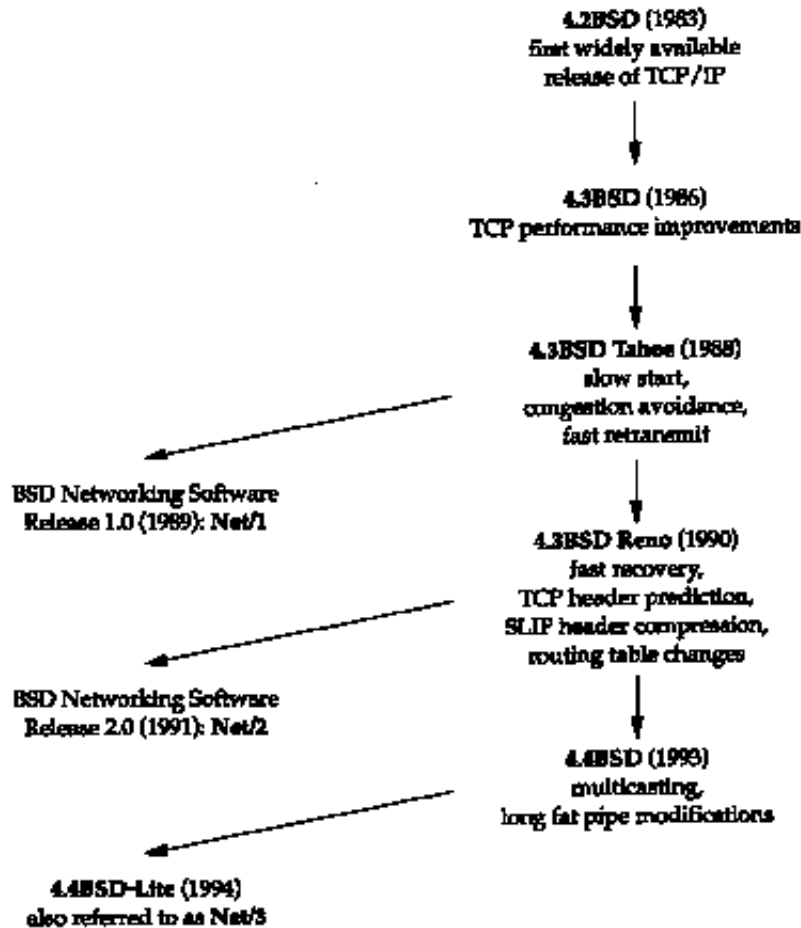
Figure 1.10 Various BSD releases with important TCP/IP features.
