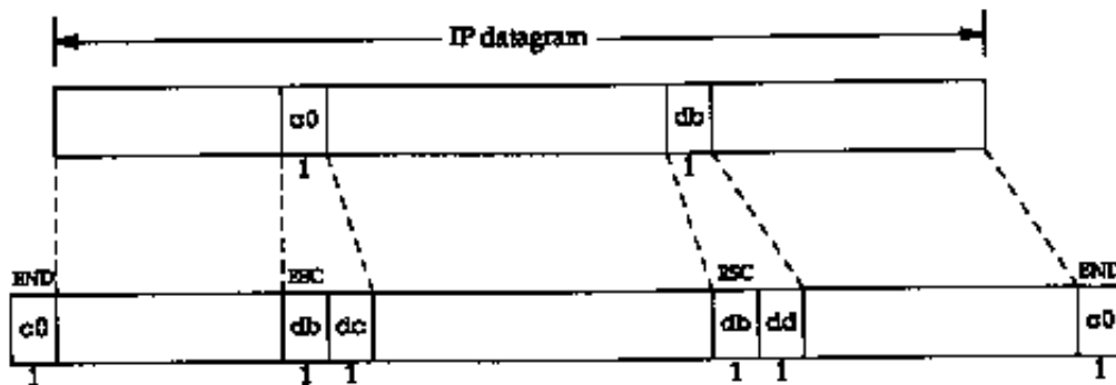
Figure 2.2 SLIP encapsulation
